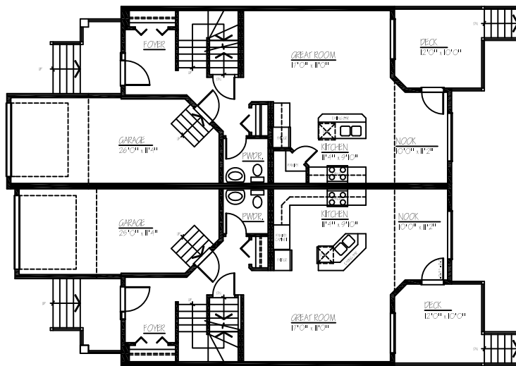
MAIN FLOOR PLAN - 711 SQ. FT. - PER UNIT
