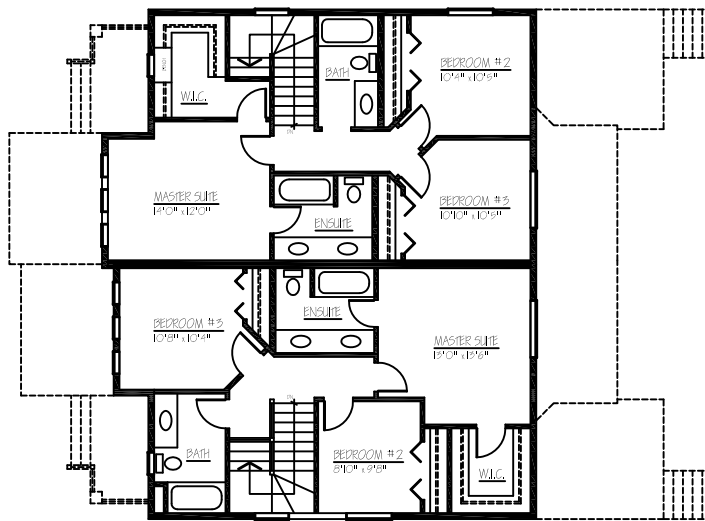
UPPER FLOOR PLAN - 709 SQ. FT. - PER UNIT
